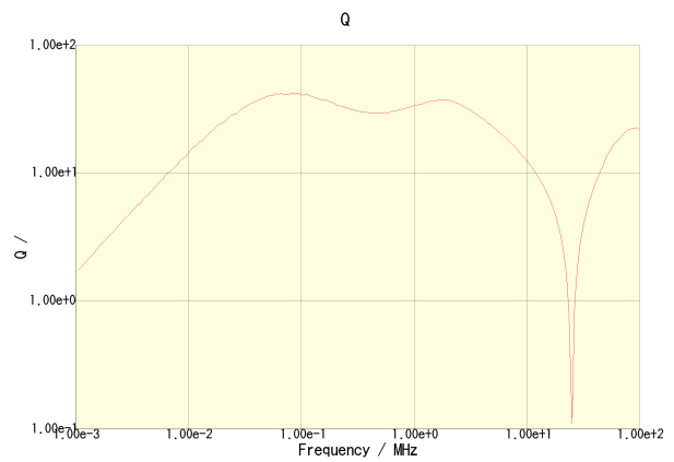
CLF6045T-150M-CA
