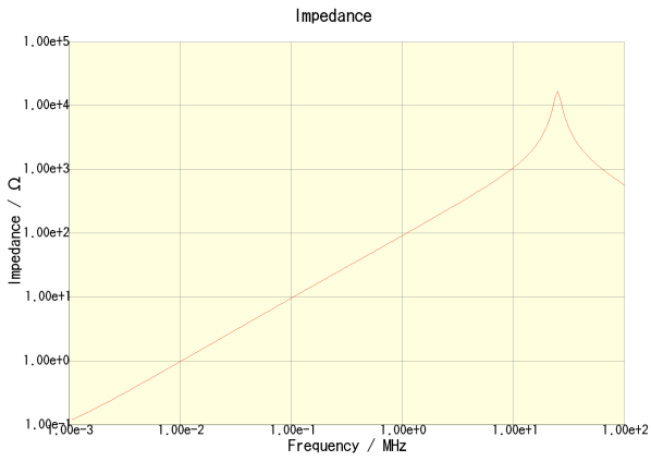
CLF6045T-150M-CA
