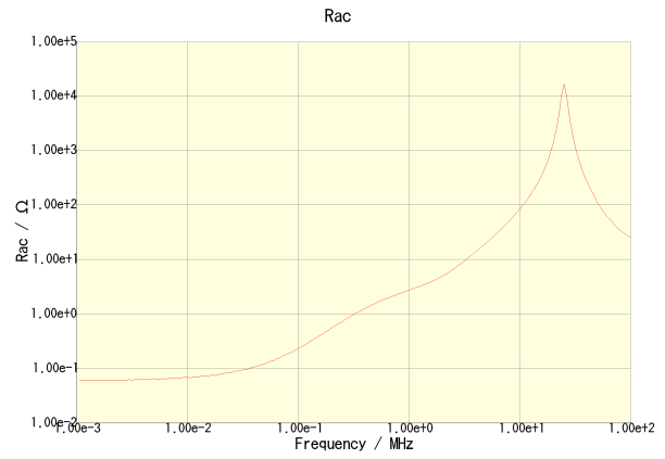
CLF6045T-150M-CA
