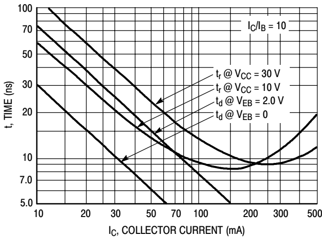
Figure 5. Turn-On Time
