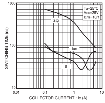
Fig.9 Switching Time
