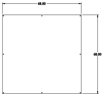
INNER PANEL
