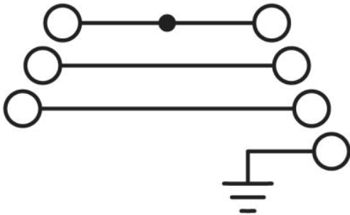
Circuit diagram
