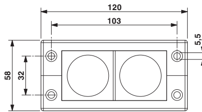
Dimensioned drawing
