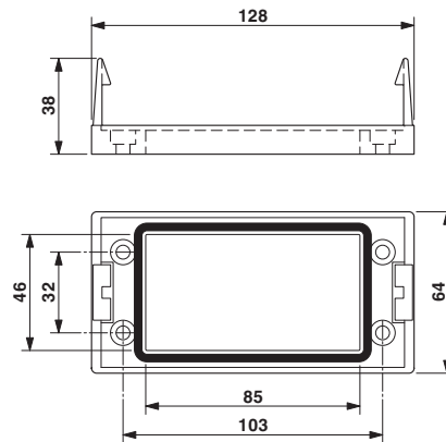
Dimensioned drawing
