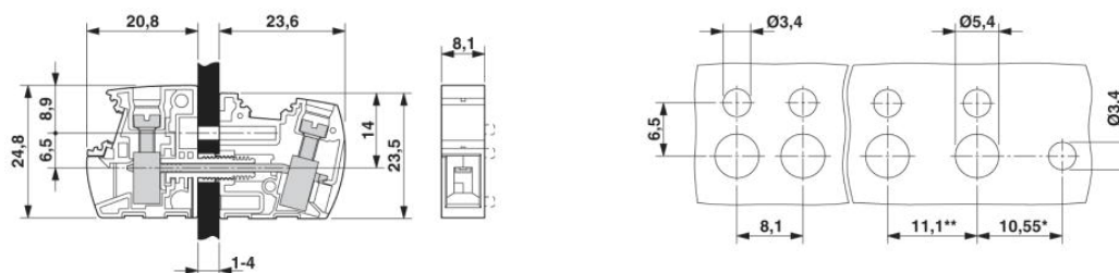
Dimensioned drawing
