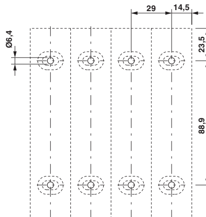
Dimensional drawing
