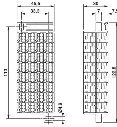
Dimensional drawing
