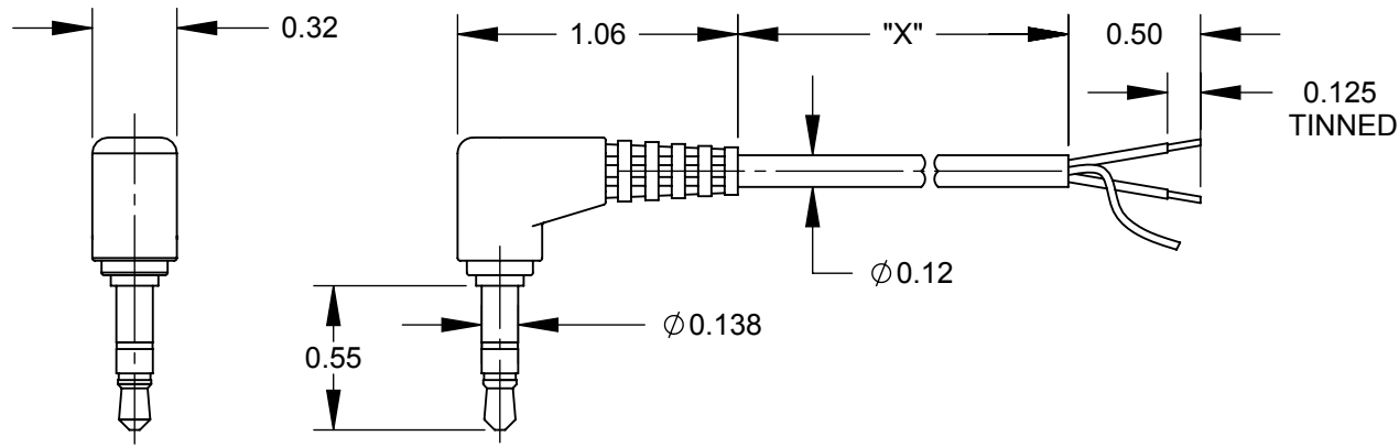
3.5 STEREO PLUG
