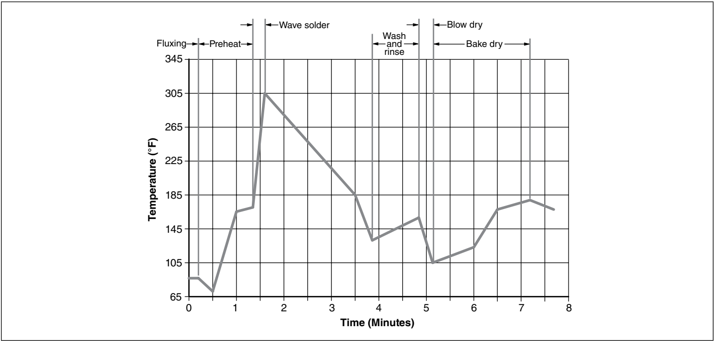
Figure 2. Recommended Wave Solder and Board Wash Parameters
