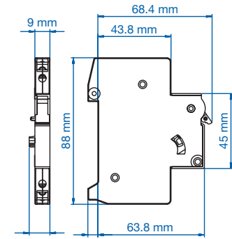
Dimensions HLS11L.
