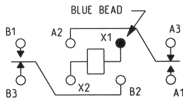
TERMINAL VIEW
