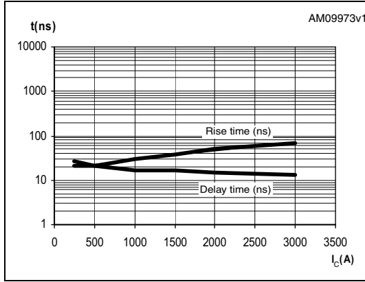
Figure 8. Resistive load switching time (ON)
