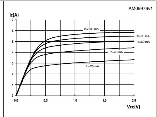
Figure 11. Output curve
