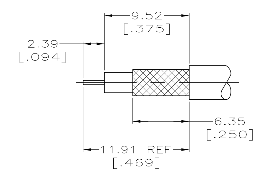
RECOMMENDED STRIP LENGTH SCALE 4:1
