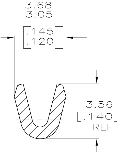
SECTION A-A SCALE 8:1
