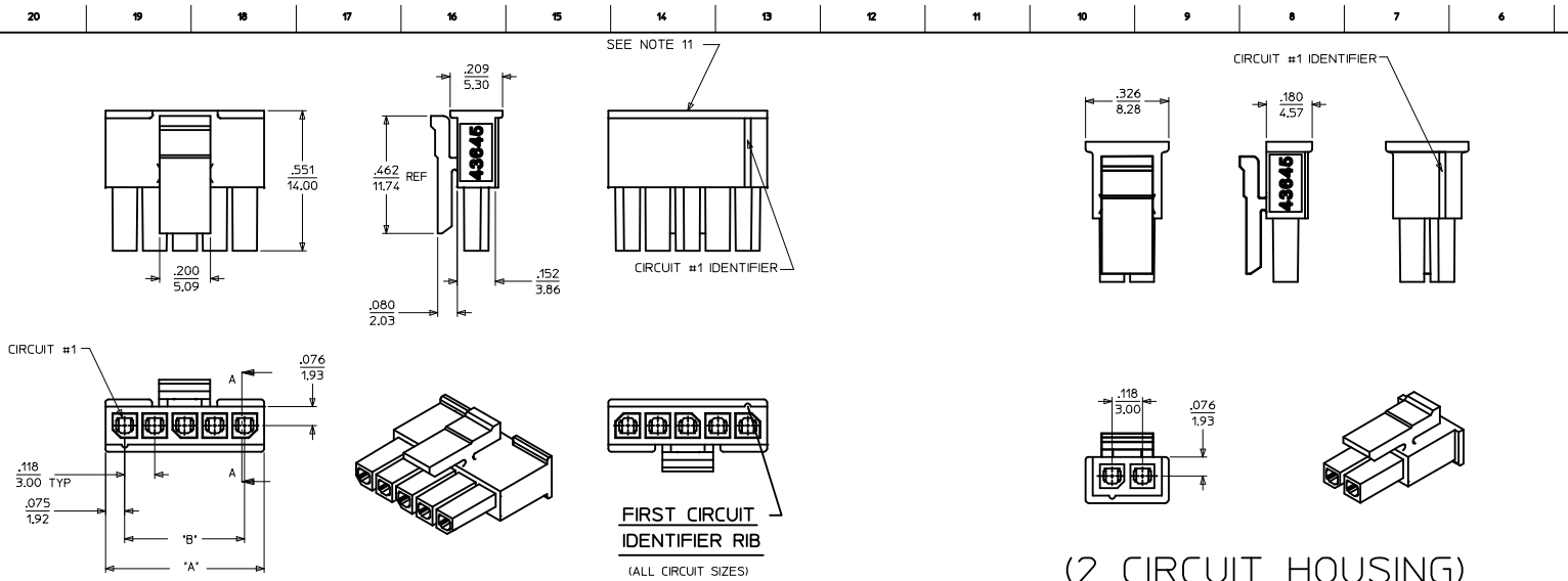
(3-12 CIRCUIT HOUSING)
