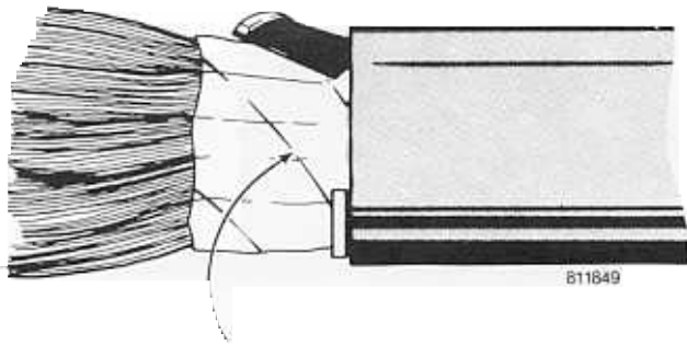
leave space for shield bond connector
