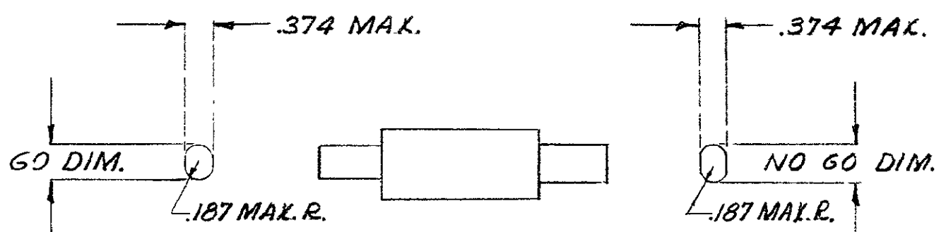
SUGGESTED PLUG GAGE DESIGN
