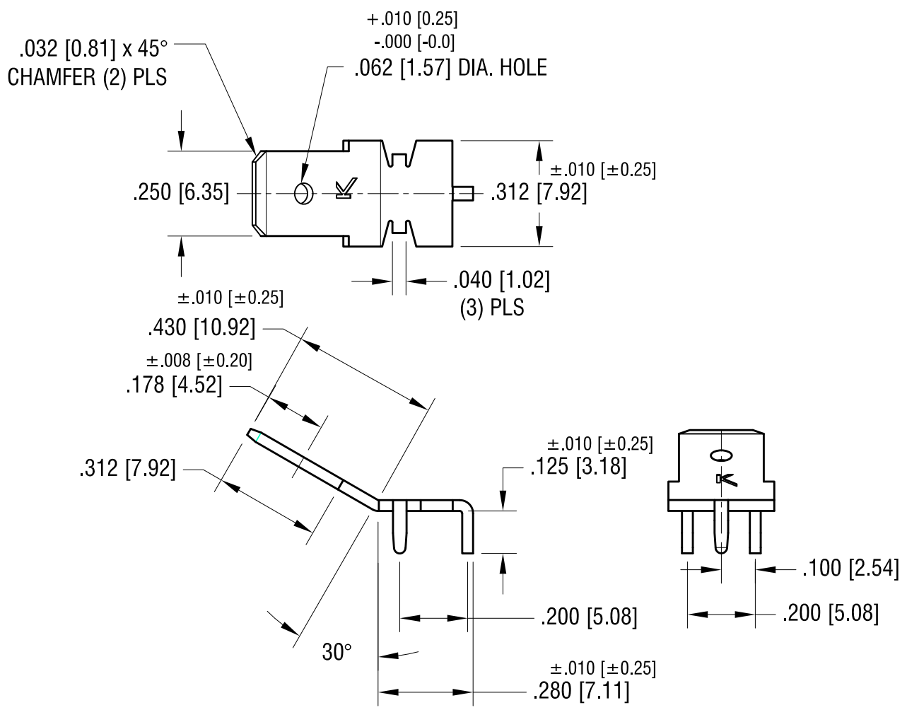
MOUNTING DETAIL
