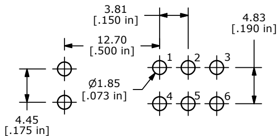
PC MOUNTING
