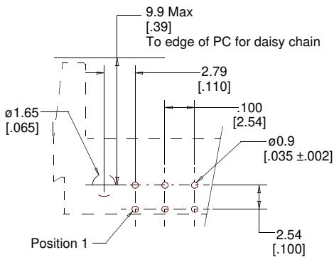
Recommended Mounting Hole Pattern
