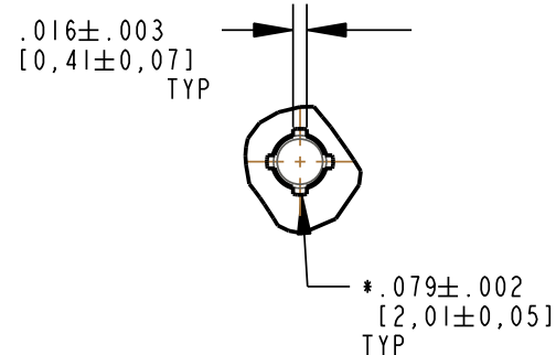
DETAIL A SCALE 4.000
