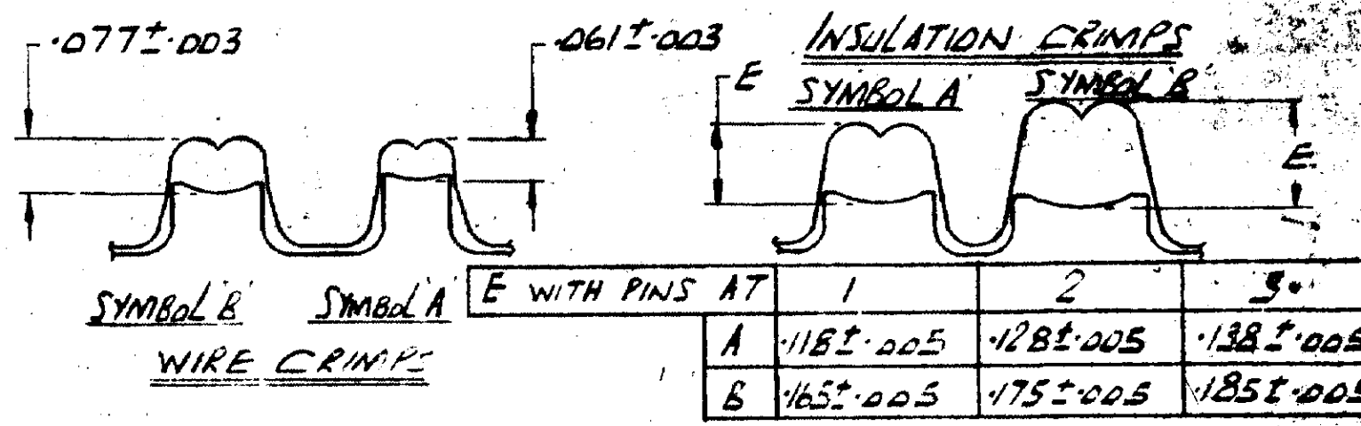
ENLARGED VIEWS ON CRIMPS SCALE: -4:1
