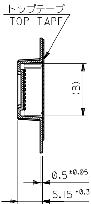
SECT. Y-Y
