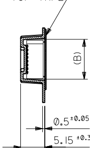
SECT. Z-Z
