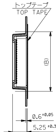
SECT. Z-Z
