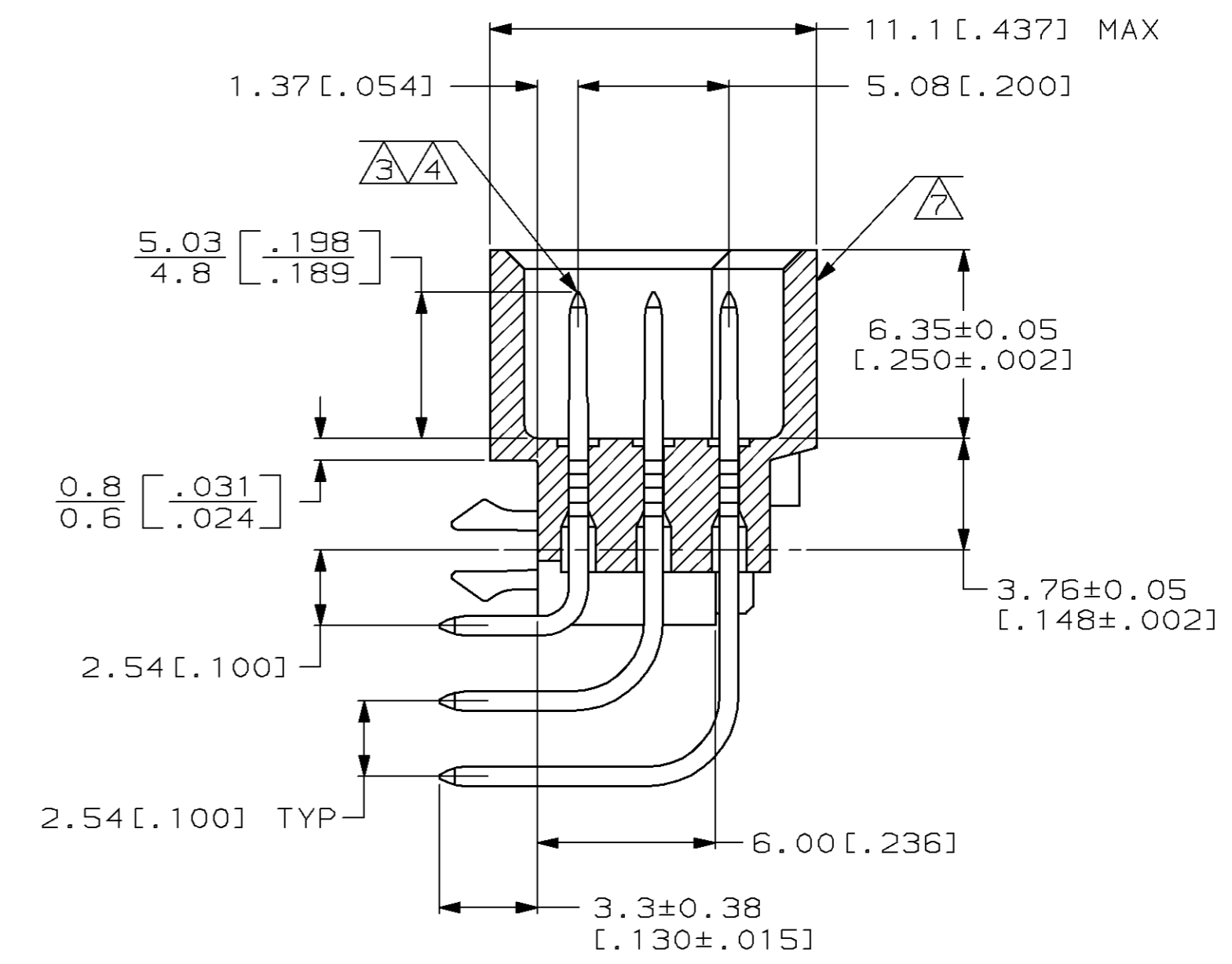
SECTION X-X
