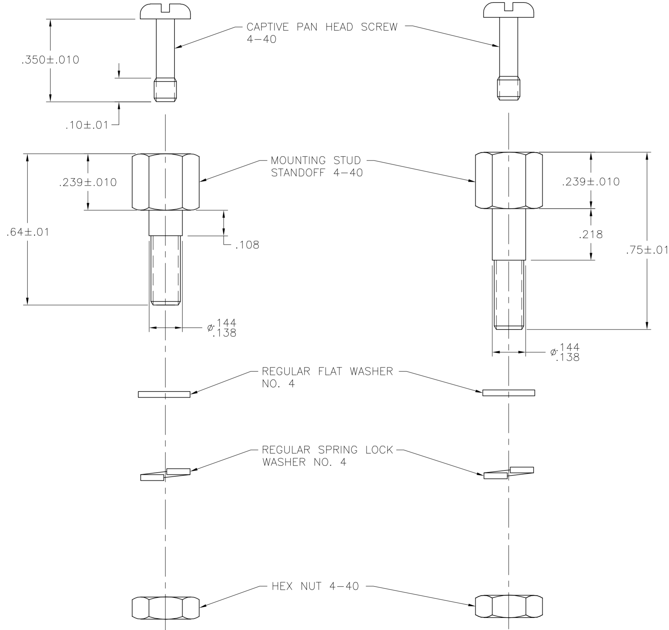
KIT P/N 5552568-2 VIEW B
