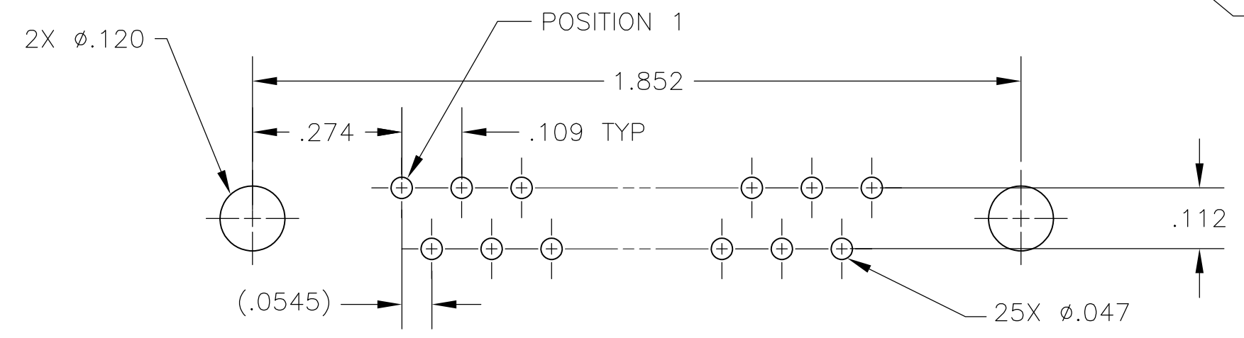
P.C. BOARD MOUNTING DIMENSIONS
