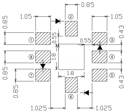
Solder pattern
