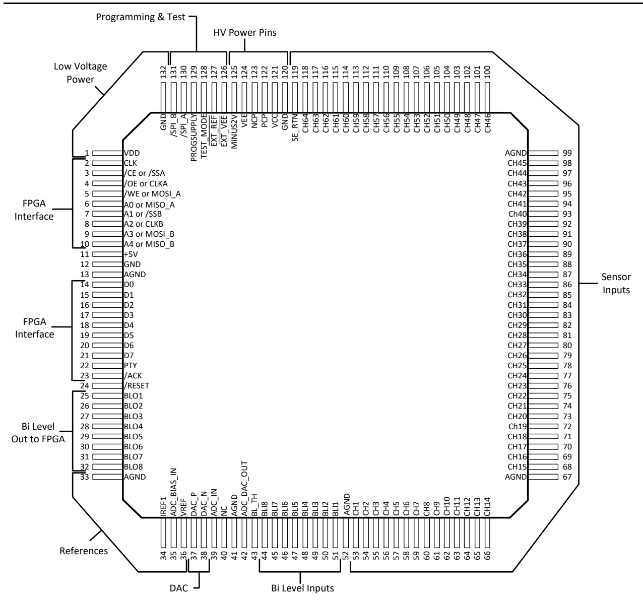
Figure 2 · Pinout
