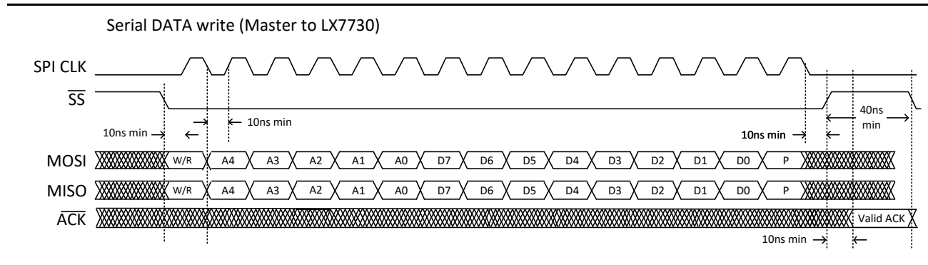
Figure 6 · Serial Data Write Timing Diagram
