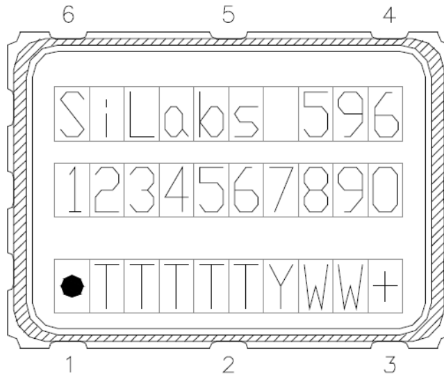
Figure 6. Mark Specification Table 16. Si596 Top Mark Description
