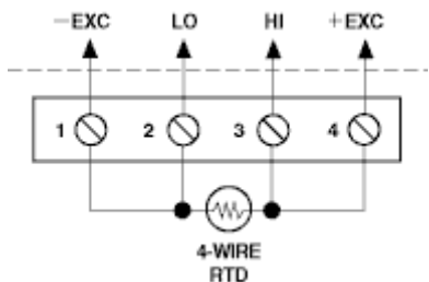
Figure 3 5B35 Input Field Connections
