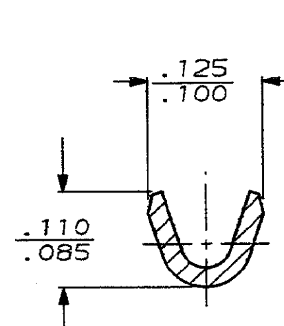
SECTION A-A SCALE 8:1
