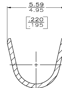
SECTION B-B SCALE 10:1
