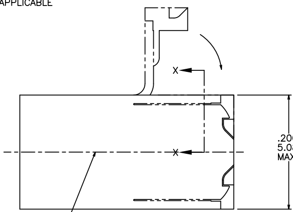
BONDED SEAM (OPTIONAL)
