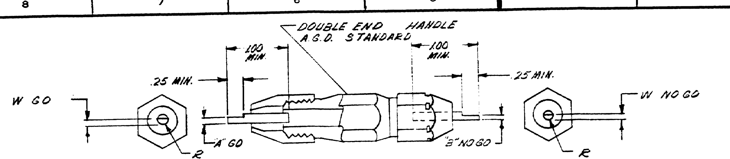
SUGGESTED PLUG GAGE DESIGN FOR "W" CRIMP
