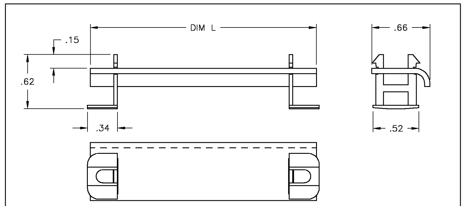
ASSEMBLED VIEW
