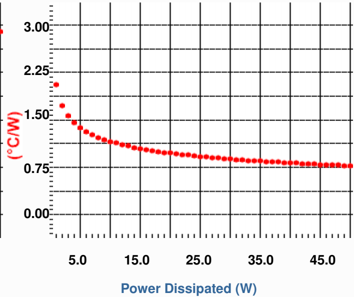
Heat Sink Thermal Resistance
