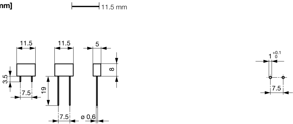
Drilling diagram
