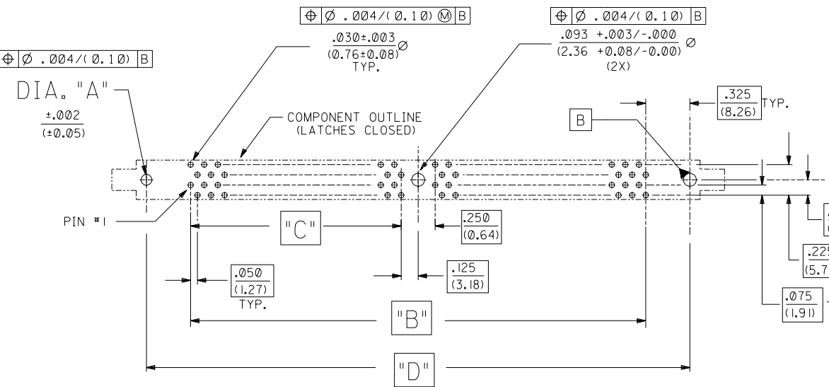
RECOMMENDED P.C. BOARD HOLE PATTERN (CONNECTOR SIDE)
