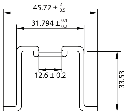
CLIP 1.80 ± 0.03mm Dia. Stainless Steel Wire
