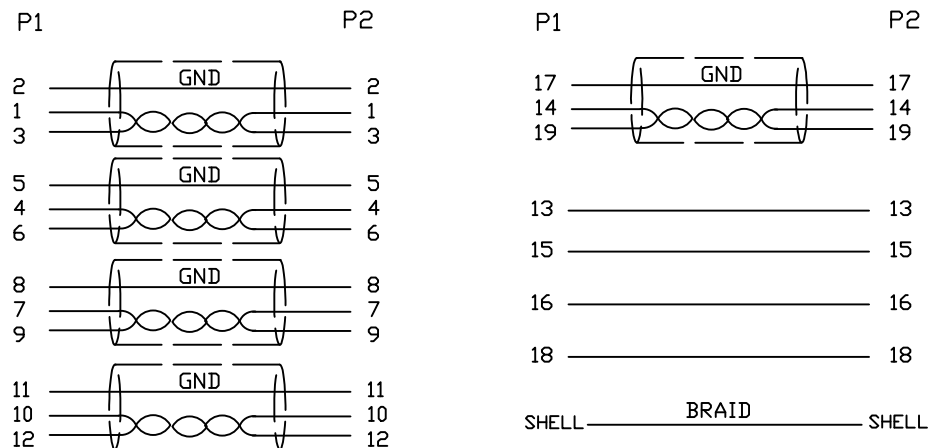
1.Wiring Diagram.
