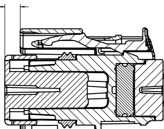
PRIMARY LOCK REINFORCEMENT (PLR) SHOWN IN PRE-STAGED POSITION
