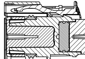
PRIMARY LOCK REINFORCEMENT (PLR) SHOWN IN FINAL-LOCK POSITION
