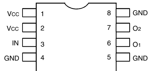
SOIC TOP VIEW
