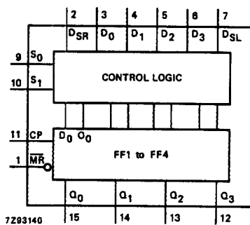
Fig.4 Functional diagram.
