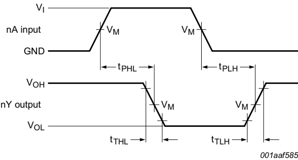
Measurement points are given in Table 10 . V_{\text{OL}} and V_{\text{OH}} are typical output voltage levels that occur with the output load.
