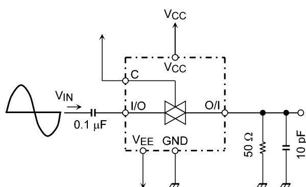
Figure 3 Frequency Response
