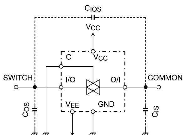
Figure 2 C_{1OS} , C_{1S} , C_{OS}
