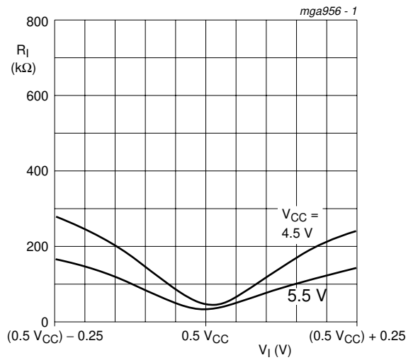
Fig 15. Input resistance at SIG_IN; COMP_IN with \Delta V_i = 0.5 V at self-bias point
