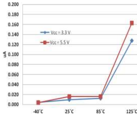
Figure 21 I S(OFF) OFF state leakage V IN = 0 V
