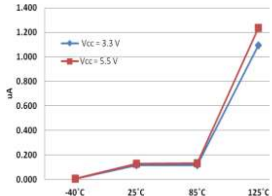
Figure 22 I S(OFF) OFF state leakage V IN = -0.1 V
